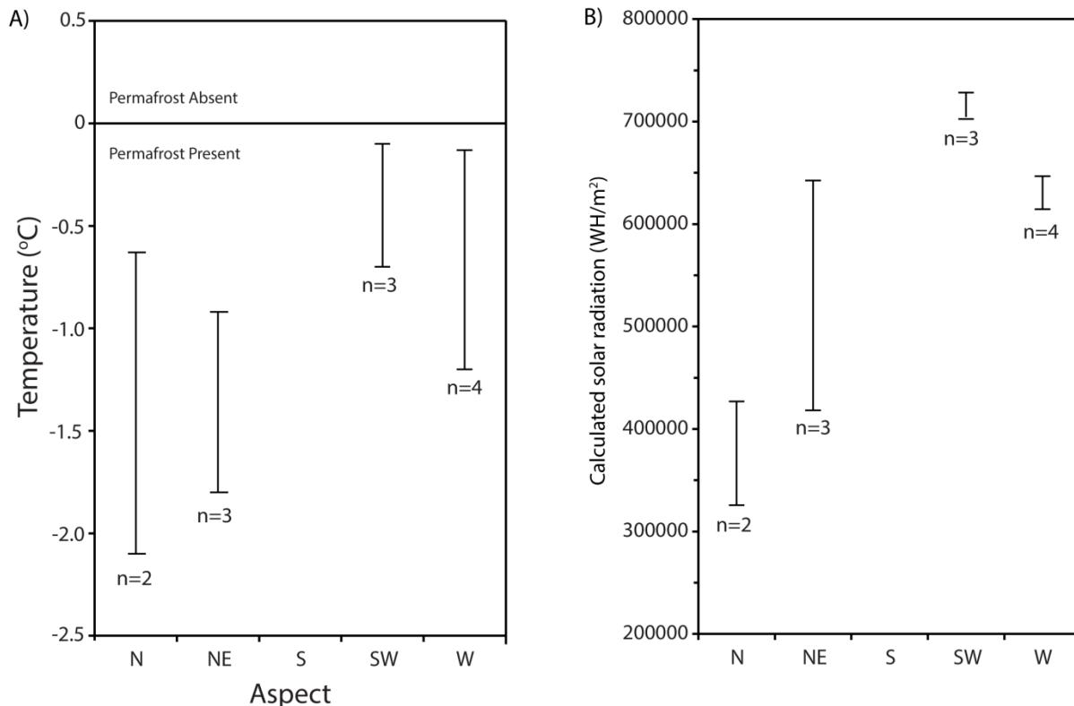
Figure 3. A) Permafrost temperature for instrumented sites with N, NE, SW and W surface aspect and B) calculated annual solar radiation.
