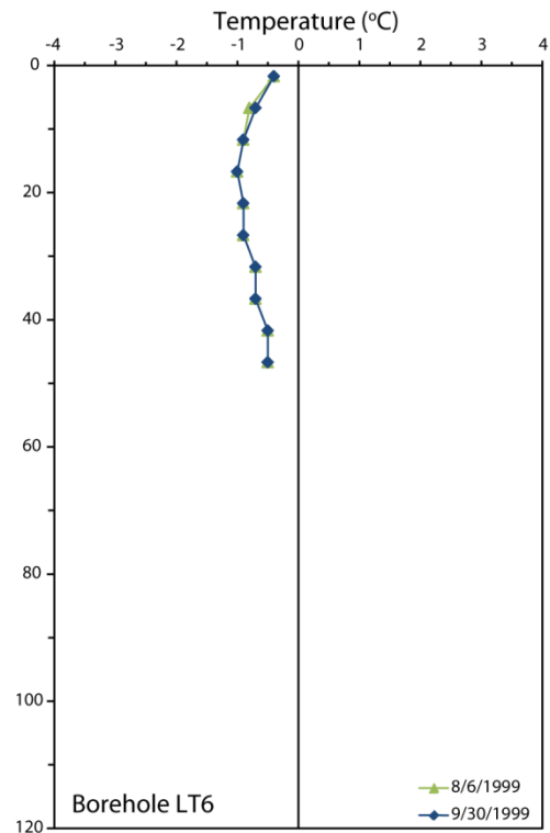
Ground temperature profiles for sites LT2, LT4, LT5 and LT6, Pogo Mine, Alaska
