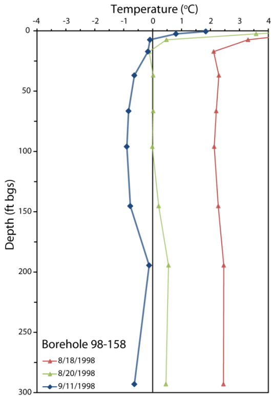
Ground temperature profiles for sites 97-42, 97-77, 98-158, 98-81, Pogo Mine, Alaska
