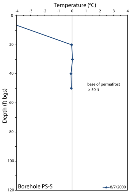
Ground temperature profiles for sites LD4, LD6, PS-5, Pogo Mine, Alaska.
