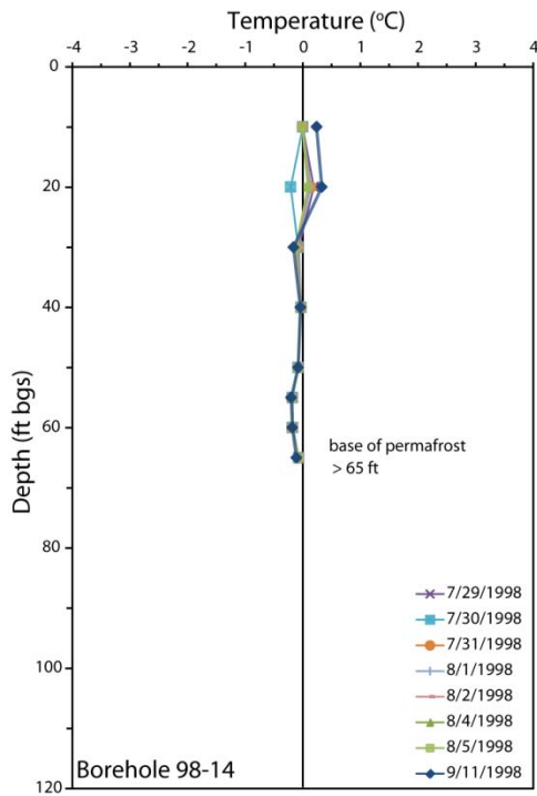
Ground temperature profiles for sites 98-12, 98-13, 98-14, Pogo Mine, Alaska
